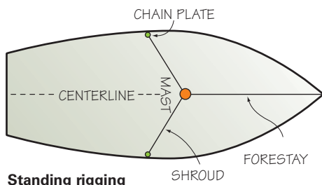
Standing rigging
